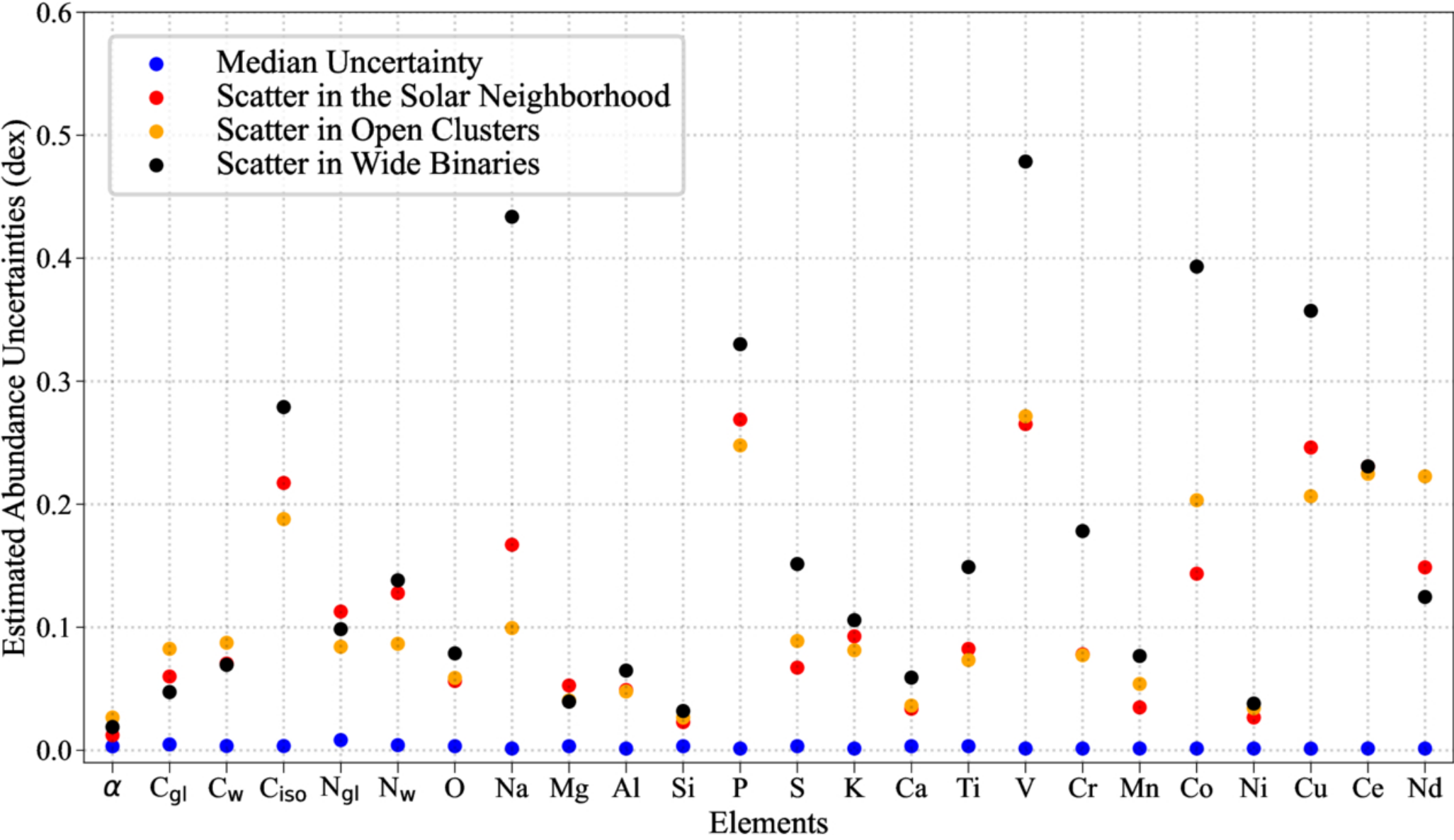
Figure 16. from Szabolcs Mészáros et al 2025 Astron. J. 170 doi:10.3847/1538-3881/ade4b9 https://dx.doi.org/10.3847/1538-3881/ade4b9 © 2025. The Author(s). Published by the American Astronomical Society.
