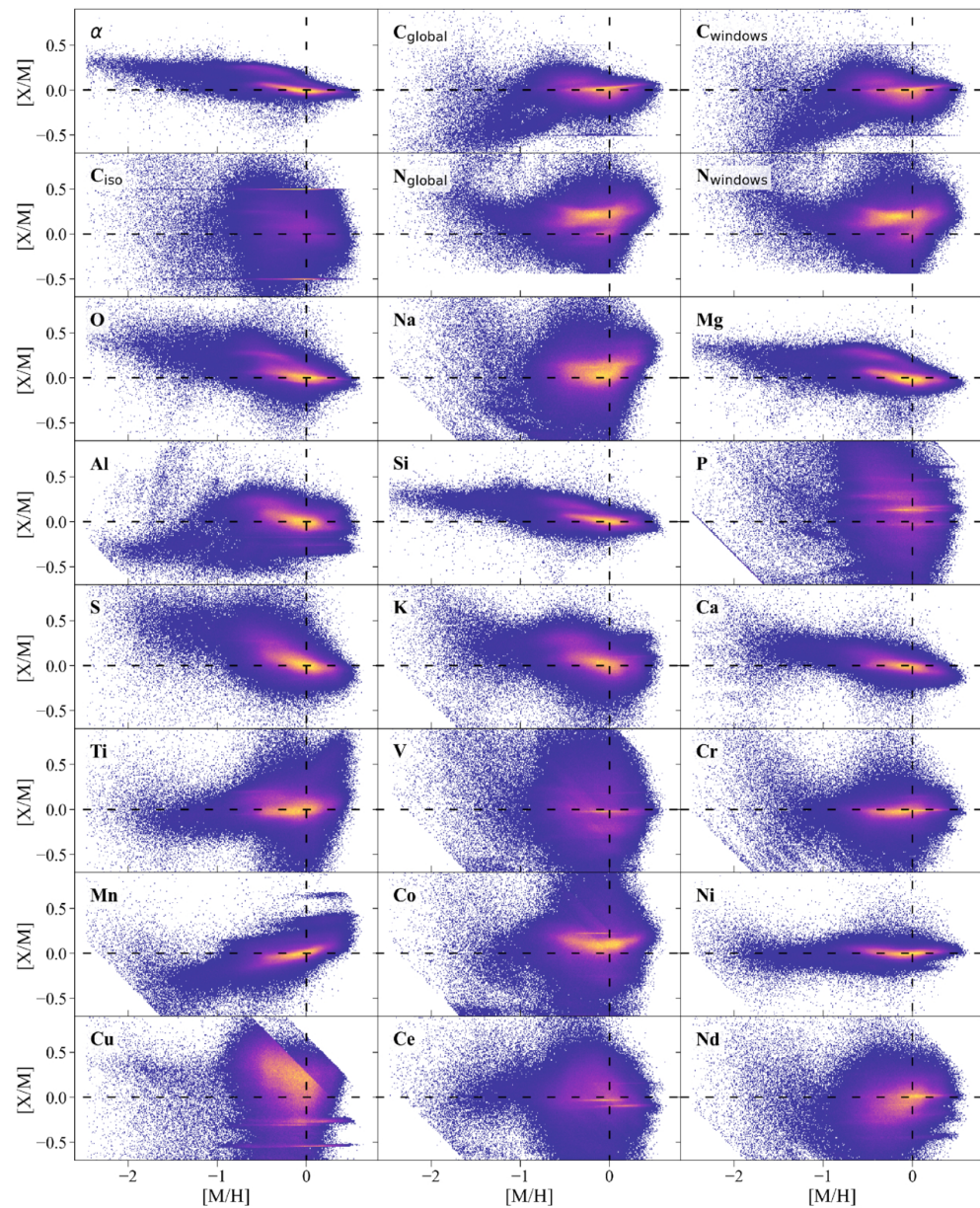
Figure 14. from Szabolcs Mészáros et al 2025 Astron. J. 170 doi:10.3847/1538-3881/ade4b9 https://dx.doi.org/10.3847/1538-3881/ade4b9 © 2025. The Author(s). Published by the American Astronomical Society.
