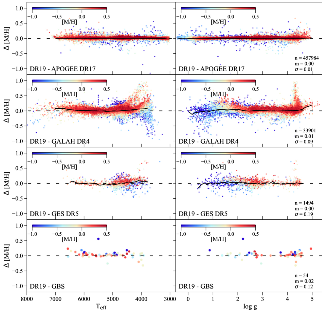
Figure 10. from Szabolcs Mészáros et al 2025 Astron. J. 170 doi:10.3847/1538-3881/ade4b9 https://dx.doi.org/10.3847/1538-3881/ade4b9 © 2025. The Author(s). Published by the American Astronomical Society.
