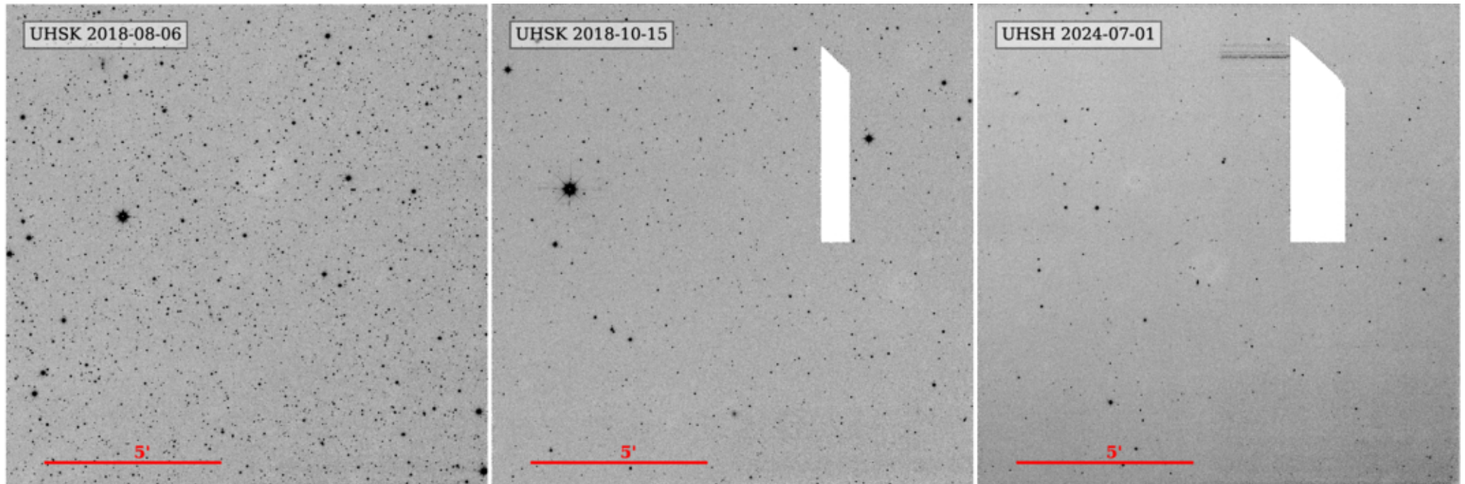
Figure 5. from Adam C. Schneider et al 2025 Astron. J. 170 doi:10.3847/1538-3881/ade43c https://dx.doi.org/10.3847/1538-3881/ade43c © 2025. The Author(s). Published by the American Astronomical Society.
