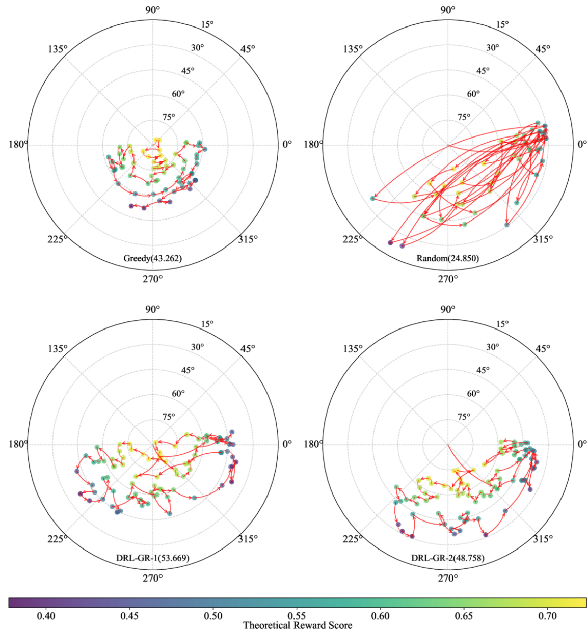
Figure 8. from Hai Cao et al 2025 Astron. J. 170 doi:10.3847/1538-3881/ade3dc https://dx.doi.org/10.3847/1538-3881/ade3dc © 2025. The Author(s). Published by the American Astronomical Society.
