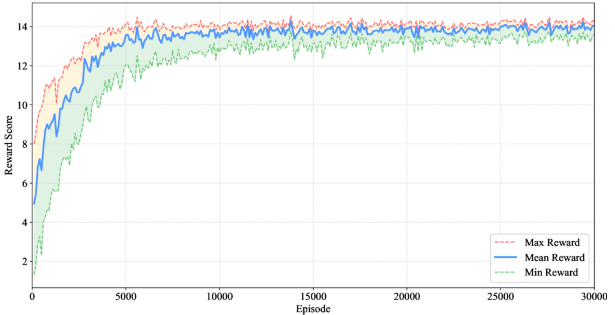
Figure 5. from Hai Cao et al 2025 Astron. J. 170 doi:10.3847/1538-3881/ade3dc https://dx.doi.org/10.3847/1538-3881/ade3dc © 2025. The Author(s). Published by the American Astronomical Society.
