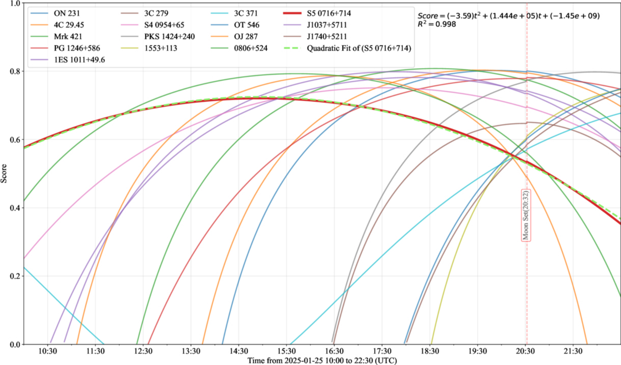
Figure 4. from Hai Cao et al 2025 Astron. J. 170 doi:10.3847/1538-3881/ade3dc https://dx.doi.org/10.3847/1538-3881/ade3dc © 2025. The Author(s). Published by the American Astronomical Society.
