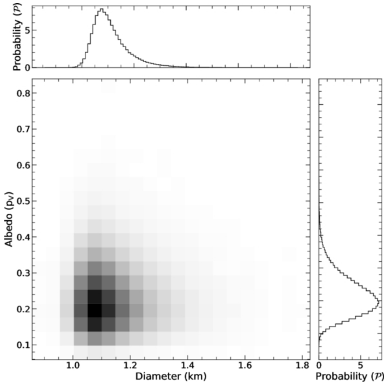
Figure 7. from Andy J. López-Oquendo et al 2025 Astron. J. 170 doi:10.3847/1538-3881/ade398 https://dx.doi.org/10.3847/1538-3881/ade398 © 2025. The Author(s). Published by the American Astronomical Society.
