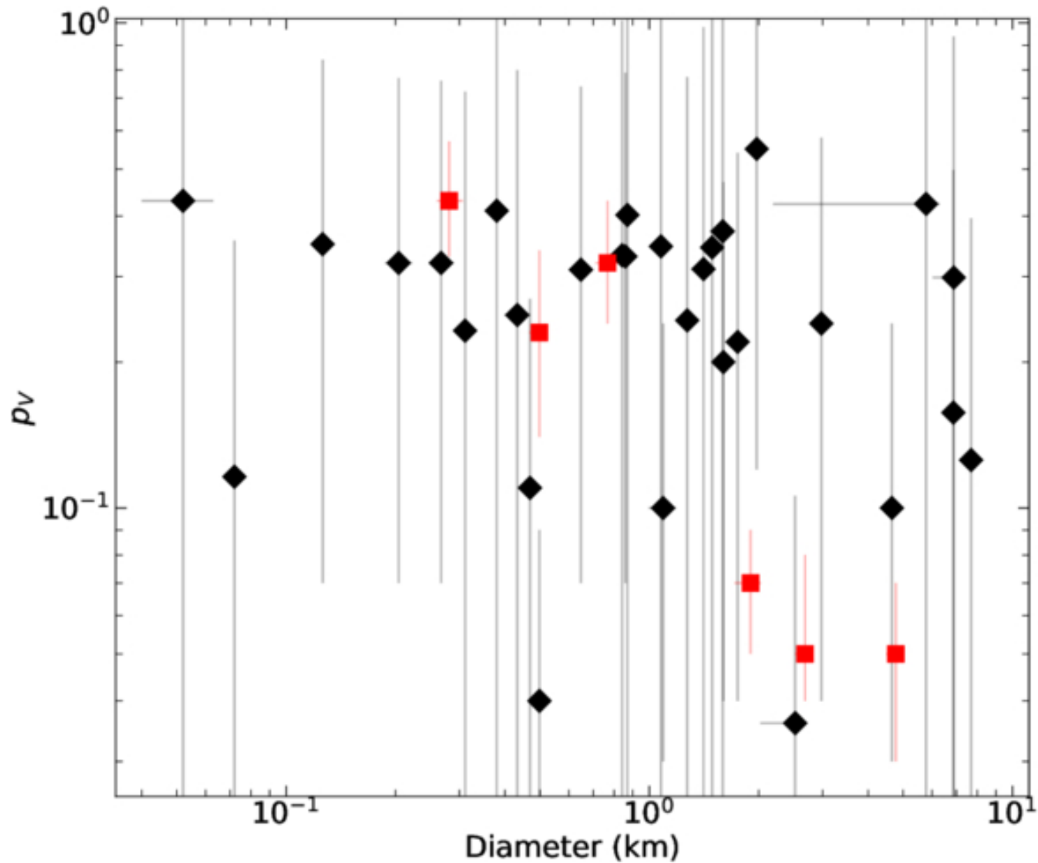
Figure 5. from Andy J. López-Oquendo et al 2025 Astron. J. 170 doi:10.3847/1538-3881/ade398 https://dx.doi.org/10.3847/1538-3881/ade398 © 2025. The Author(s). Published by the American Astronomical Society.
