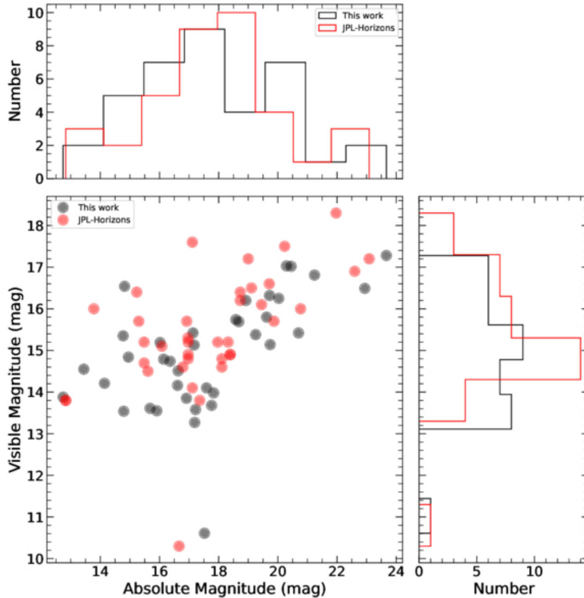
Figure 4. from Andy J. López-Oquendo et al 2025 Astron. J. 170 doi:10.3847/1538-3881/ade398 https://dx.doi.org/10.3847/1538-3881/ade398 © 2025. The Author(s). Published by the American Astronomical Society.
