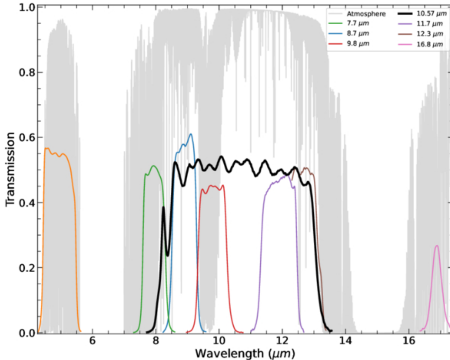
Figure 3. from Andy J. López-Oquendo et al 2025 Astron. J. 170 doi:10.3847/1538-3881/ade398 https://dx.doi.org/10.3847/1538-3881/ade398 © 2025. The Author(s). Published by the American Astronomical Society.
