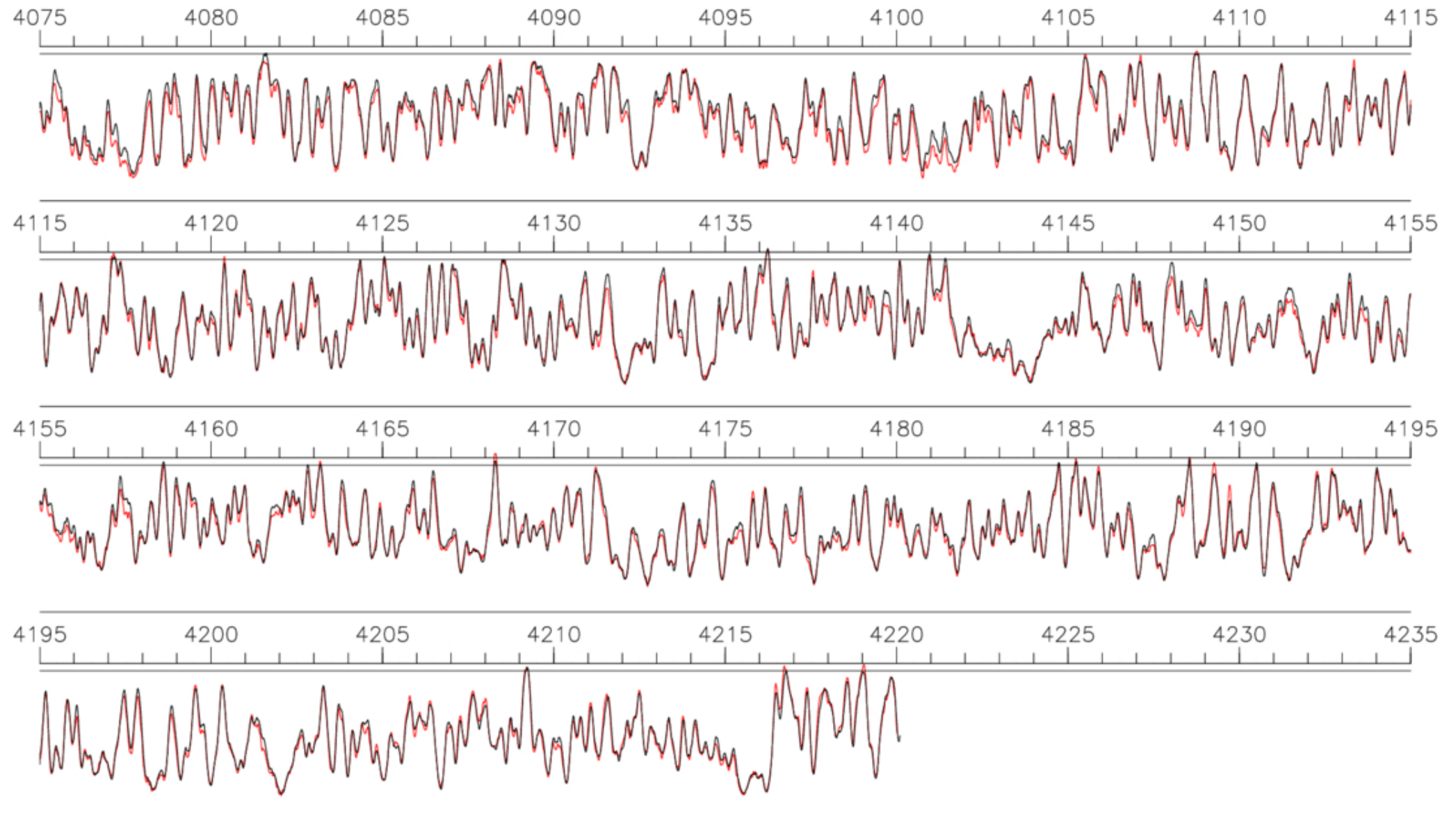
Figure 7. from Brian D. Mason et al 2025 Astron. J. 170 doi:10.3847/1538-3881/ade38d https://dx.doi.org/10.3847/1538-3881/ade38d © 2025. The Author(s). Published by the American Astronomical Society.
