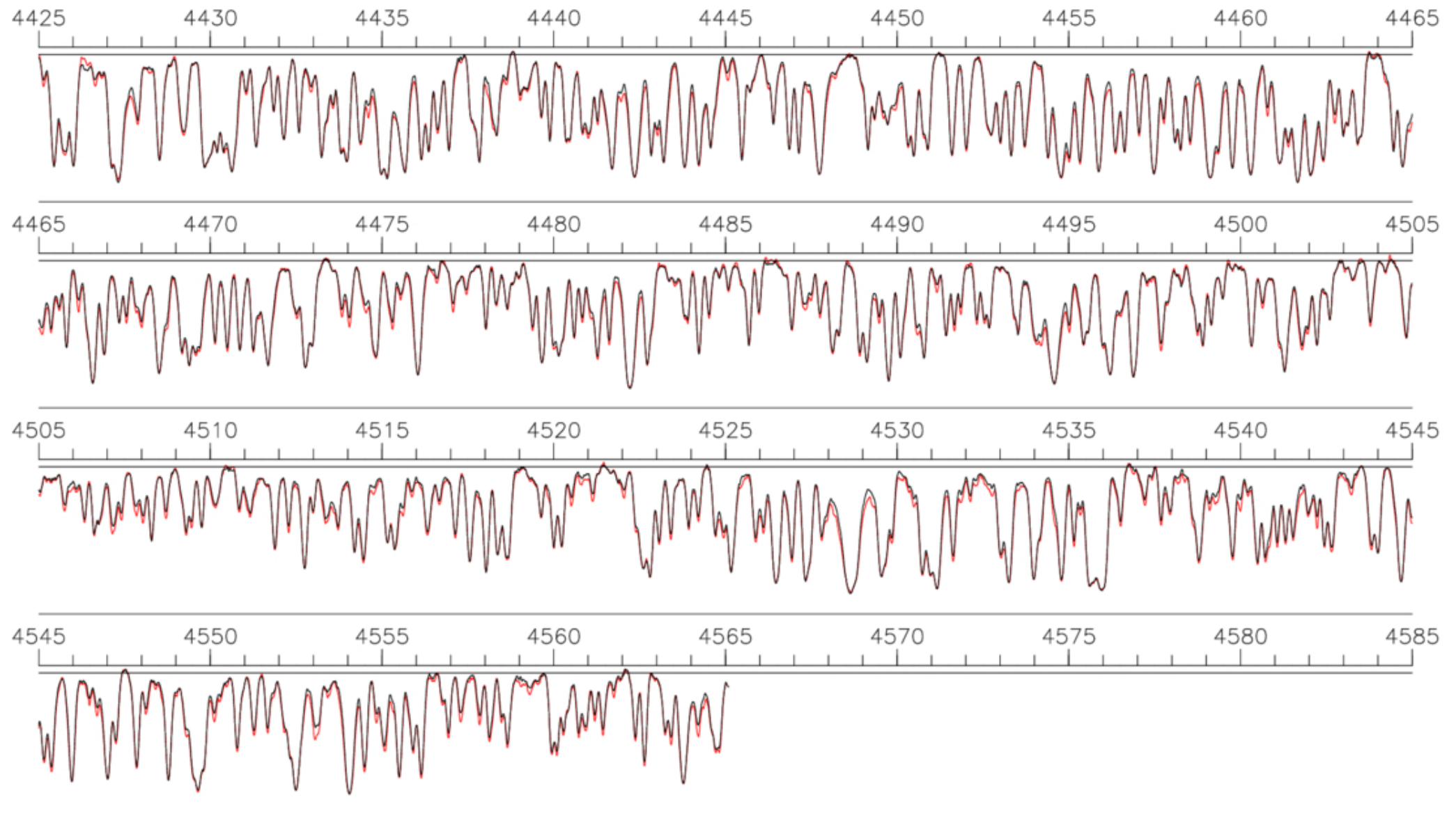
Figure 6. from Brian D. Mason et al 2025 Astron. J. 170 doi:10.3847/1538-3881/ade38d https://dx.doi.org/10.3847/1538-3881/ade38d © 2025. The Author(s). Published by the American Astronomical Society.
