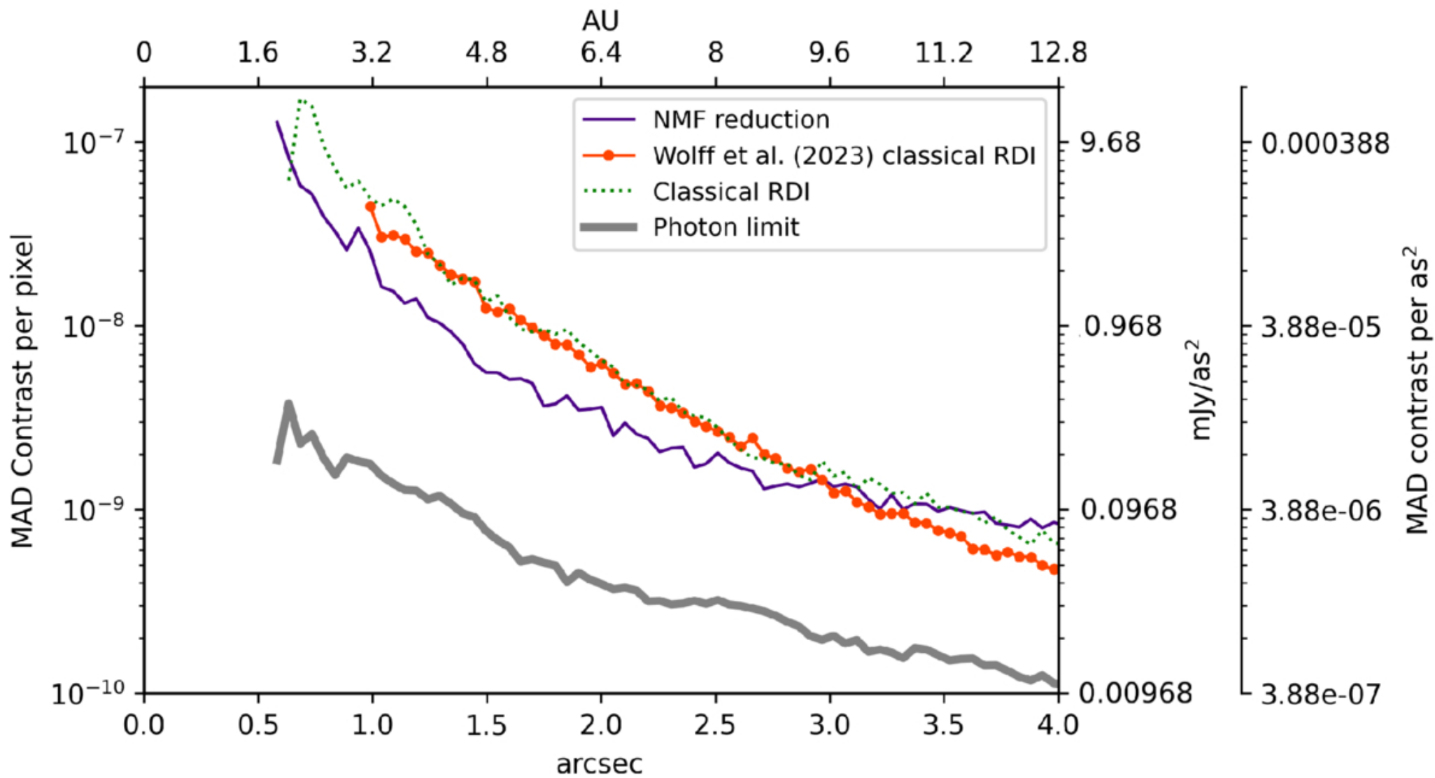
Figure 6. from Sai Krishanth P. M. et al 2025 Astron. J. 170 doi:10.3847/1538-3881/ade234 https://dx.doi.org/10.3847/1538-3881/ade234 © 2025. The Author(s). Published by the American Astronomical Society.
