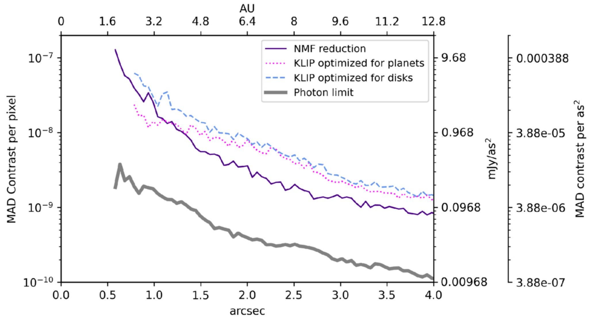
Figure 5. from Sai Krishanth P. M. et al 2025 Astron. J. 170 doi:10.3847/1538-3881/ade234 https://dx.doi.org/10.3847/1538-3881/ade234 © 2025. The Author(s). Published by the American Astronomical Society.
