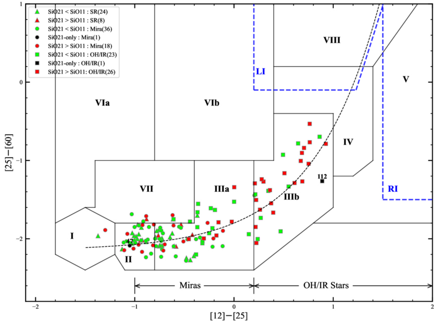
Figure 9. from Hyeon Baek et al 2025 Astron. J. 170 doi:10.3847/1538-3881/ade1d1 https://dx.doi.org/10.3847/1538-3881/ade1d1 © 2025. The Author(s). Published by the American Astronomical Society.
