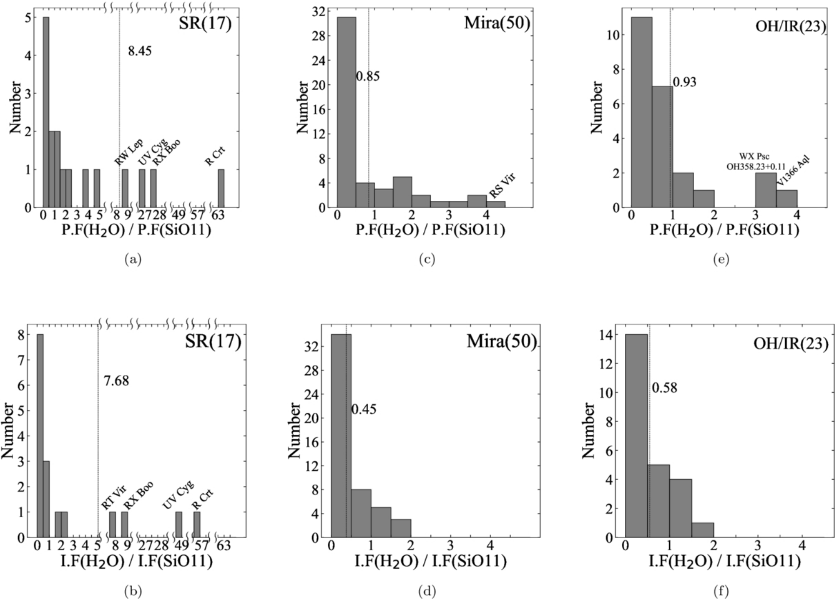
Figure 2. from Hyeon Baek et al 2025 Astron. J. 170 doi:10.3847/1538-3881/ade1d1 https://dx.doi.org/10.3847/1538-3881/ade1d1 © 2025. The Author(s). Published by the American Astronomical Society.
