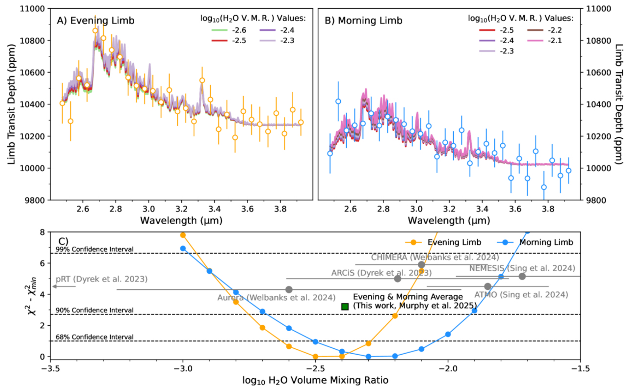
Figure 8. from Matthew M. Murphy et al 2025 Astron. J. 170 doi:10.3847/1538-3881/addf38 https://dx.doi.org/10.3847/1538-3881/addf38 © 2025. The Author(s). Published by the American Astronomical Society.
