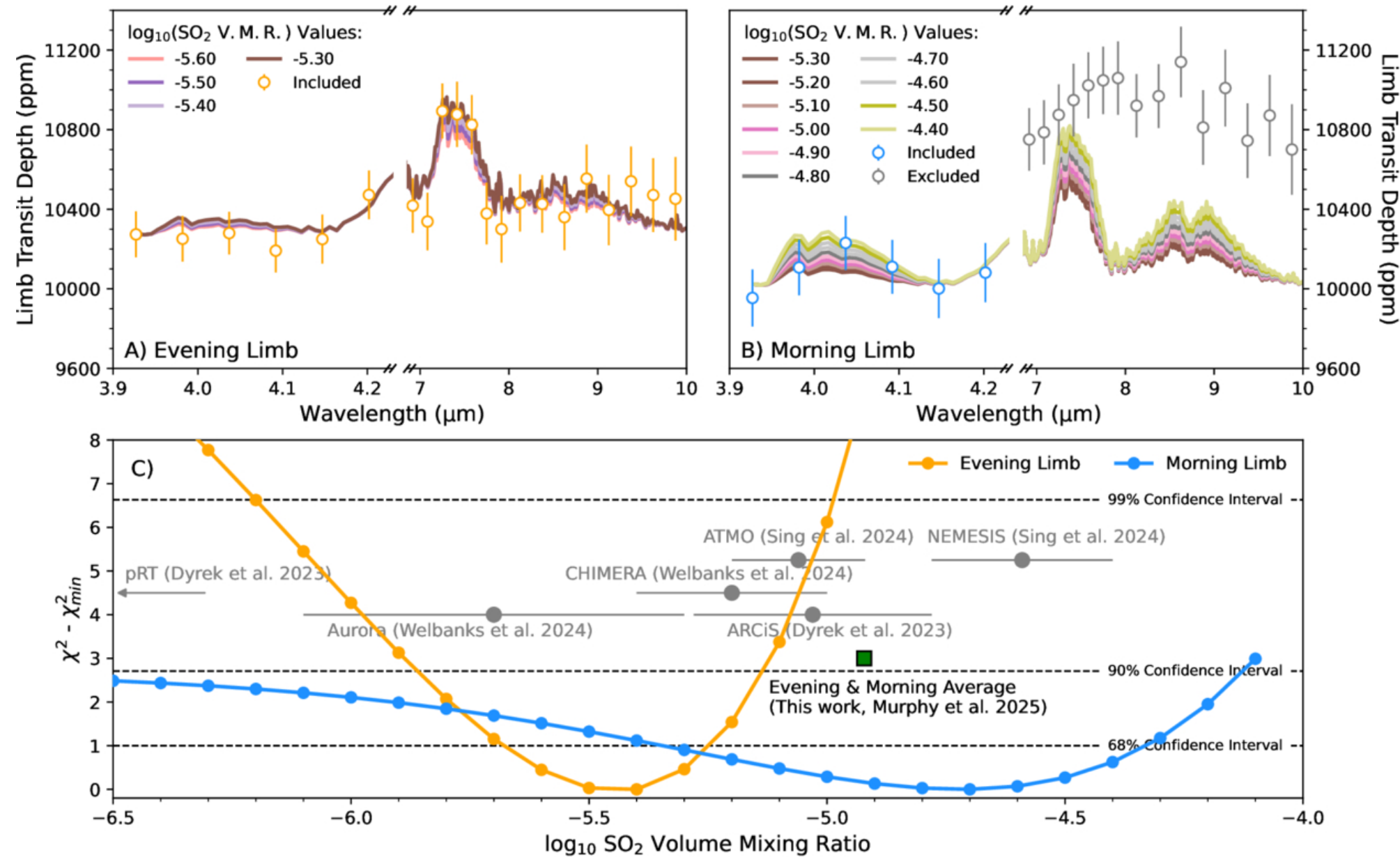
Figure 6. from Matthew M. Murphy et al 2025 Astron. J. 170 doi:10.3847/1538-3881/addf38 https://dx.doi.org/10.3847/1538-3881/addf38 © 2025. The Author(s). Published by the American Astronomical Society.
