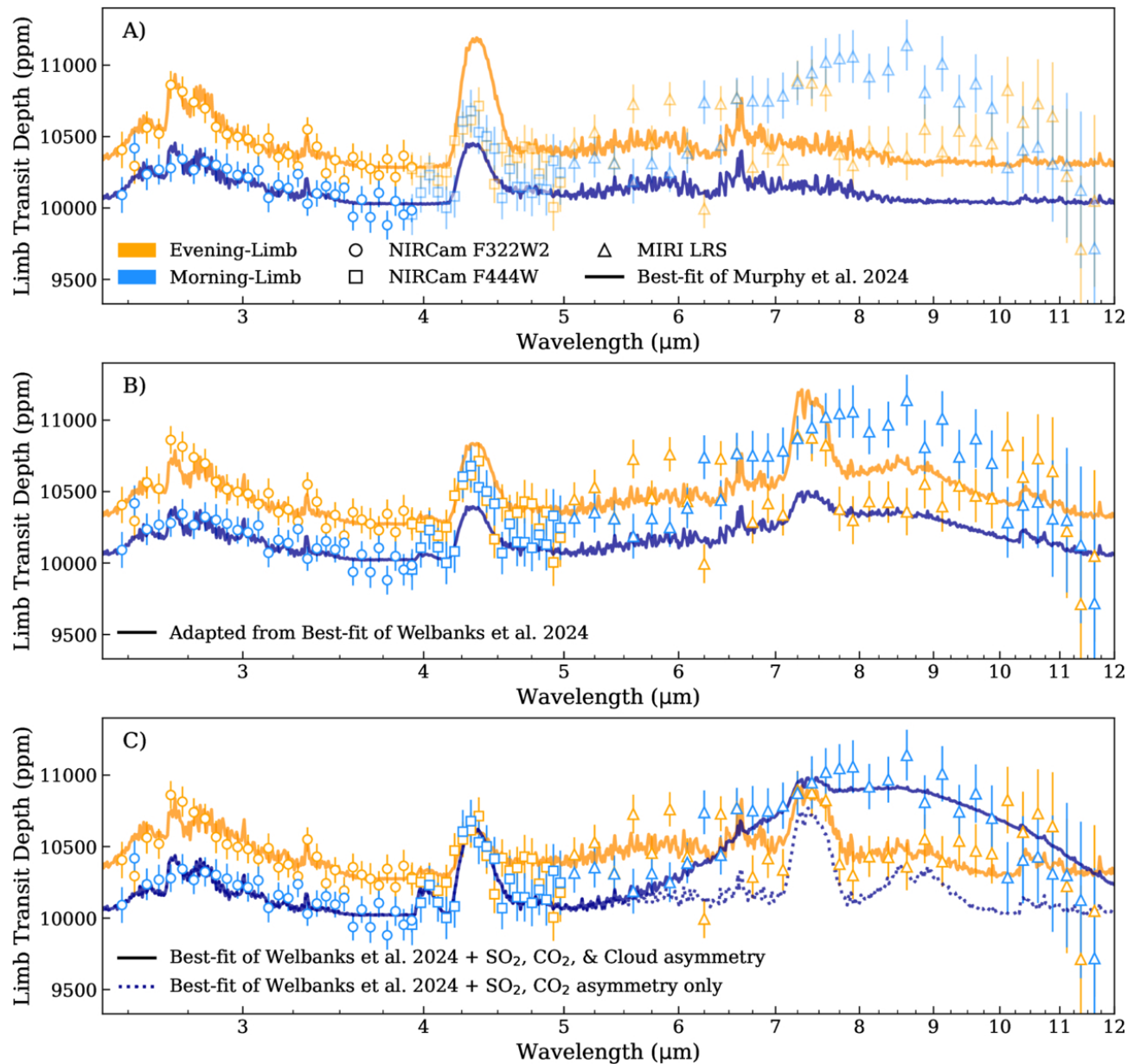
Figure 5. from Matthew M. Murphy et al 2025 Astron. J. 170 doi:10.3847/1538-3881/addf38 https://dx.doi.org/10.3847/1538-3881/addf38 © 2025. The Author(s). Published by the American Astronomical Society.
