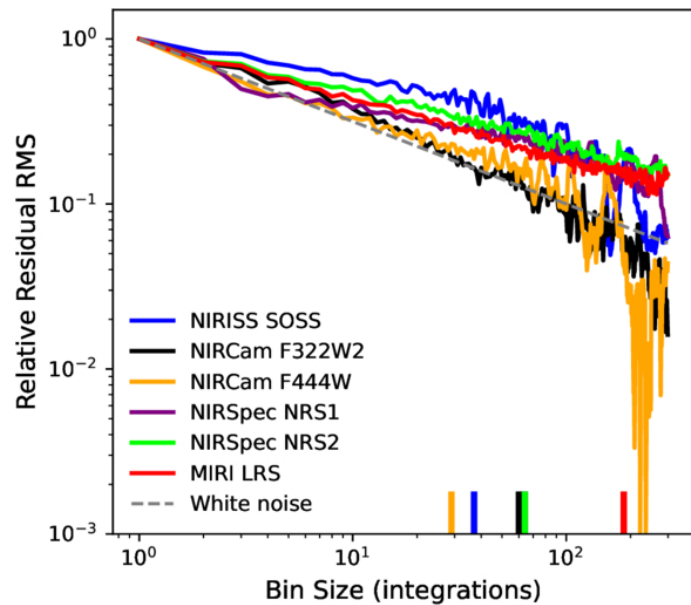
Figure 4. from Matthew M. Murphy et al 2025 Astron. J. 170 doi:10.3847/1538-3881/addf38 https://dx.doi.org/10.3847/1538-3881/addf38 © 2025. The Author(s). Published by the American Astronomical Society.
