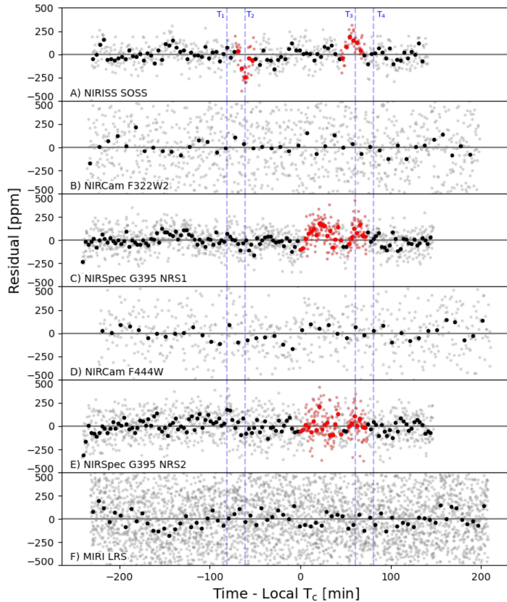
Figure 3. from Matthew M. Murphy et al 2025 Astron. J. 170 doi:10.3847/1538-3881/addf38 https://dx.doi.org/10.3847/1538-3881/addf38 © 2025. The Author(s). Published by the American Astronomical Society.
