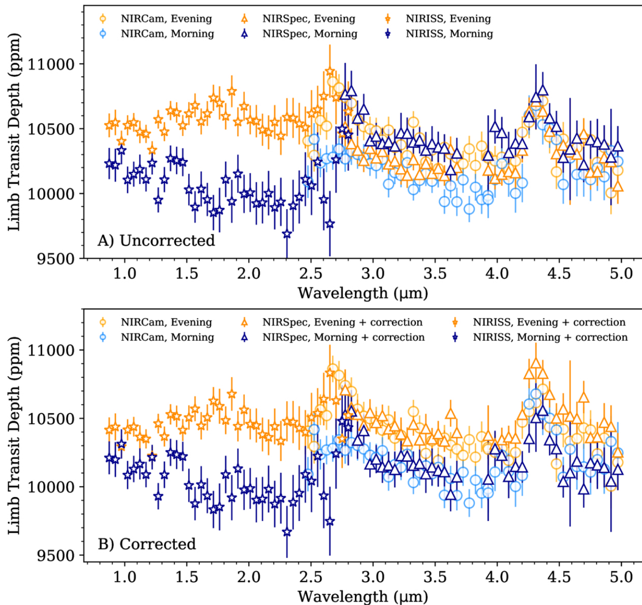
Figure 2. from Matthew M. Murphy et al 2025 Astron. J. 170 doi:10.3847/1538-3881/addf38 https://dx.doi.org/10.3847/1538-3881/addf38 © 2025. The Author(s). Published by the American Astronomical Society.
