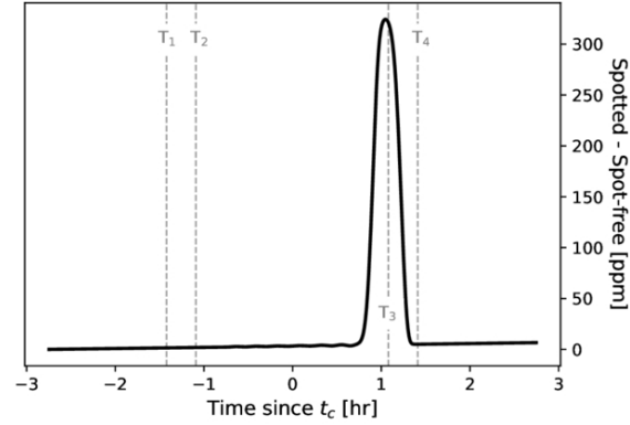
D) Crossing event strengths
