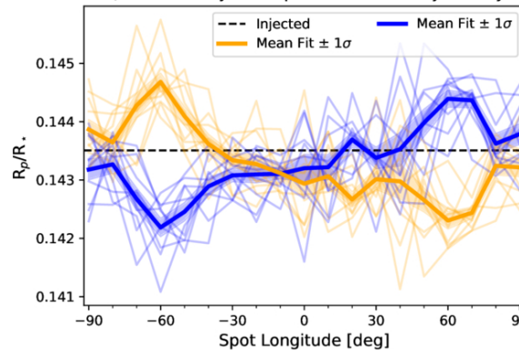
E) Control -- Injected spot but no limb asymmetry
