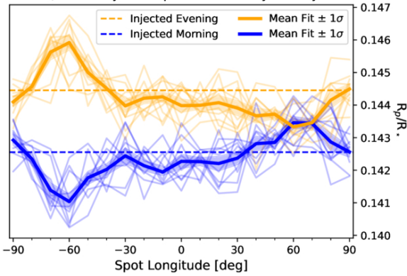
F) Test -- Injected spot and limb asymmetry
