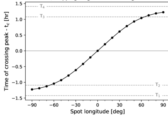
E) Control -- Injected spot but no limb asymmetry
