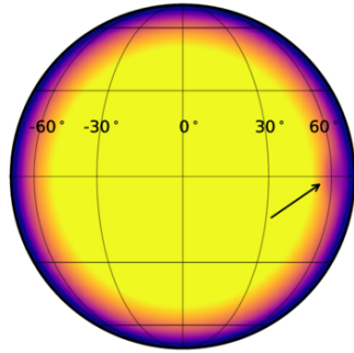
A) WASP-107 (hypothetical) spotted surface map
