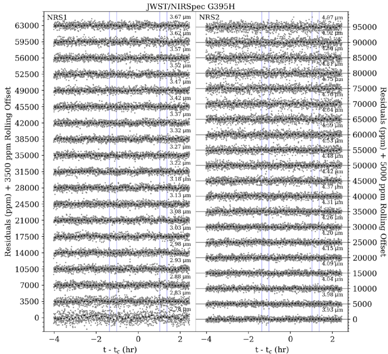
Figure B5. from Matthew M. Murphy et al 2025 Astron. J. 170 doi:10.3847/1538-3881/addf38 https://dx.doi.org/10.3847/1538-3881/addf38 © 2025. The Author(s). Published by the American Astronomical Society.
