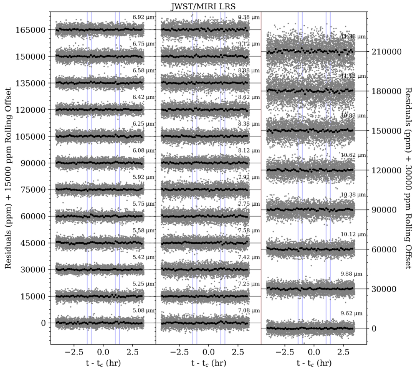
Figure B3. from Matthew M. Murphy et al 2025 Astron. J. 170 doi:10.3847/1538-3881/addf38 https://dx.doi.org/10.3847/1538-3881/addf38 © 2025. The Author(s). Published by the American Astronomical Society.
