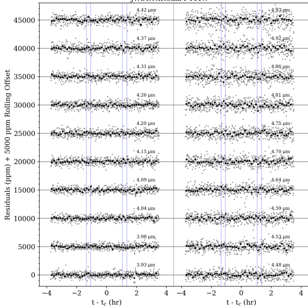
JWST/NIRCam F444W
