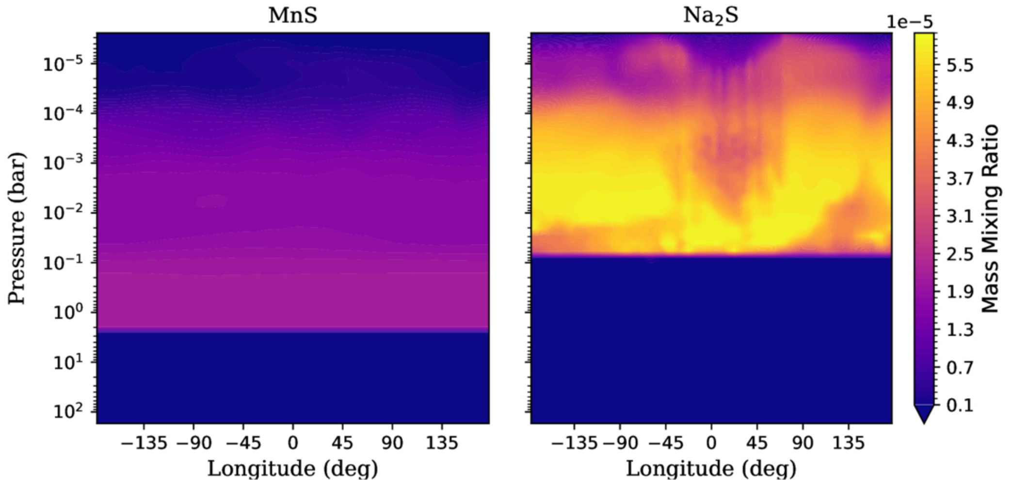
Figure 10. from Matthew M. Murphy et al 2025 Astron. J. 170 doi:10.3847/1538-3881/addf38 https://dx.doi.org/10.3847/1538-3881/addf38 © 2025. The Author(s). Published by the American Astronomical Society.
