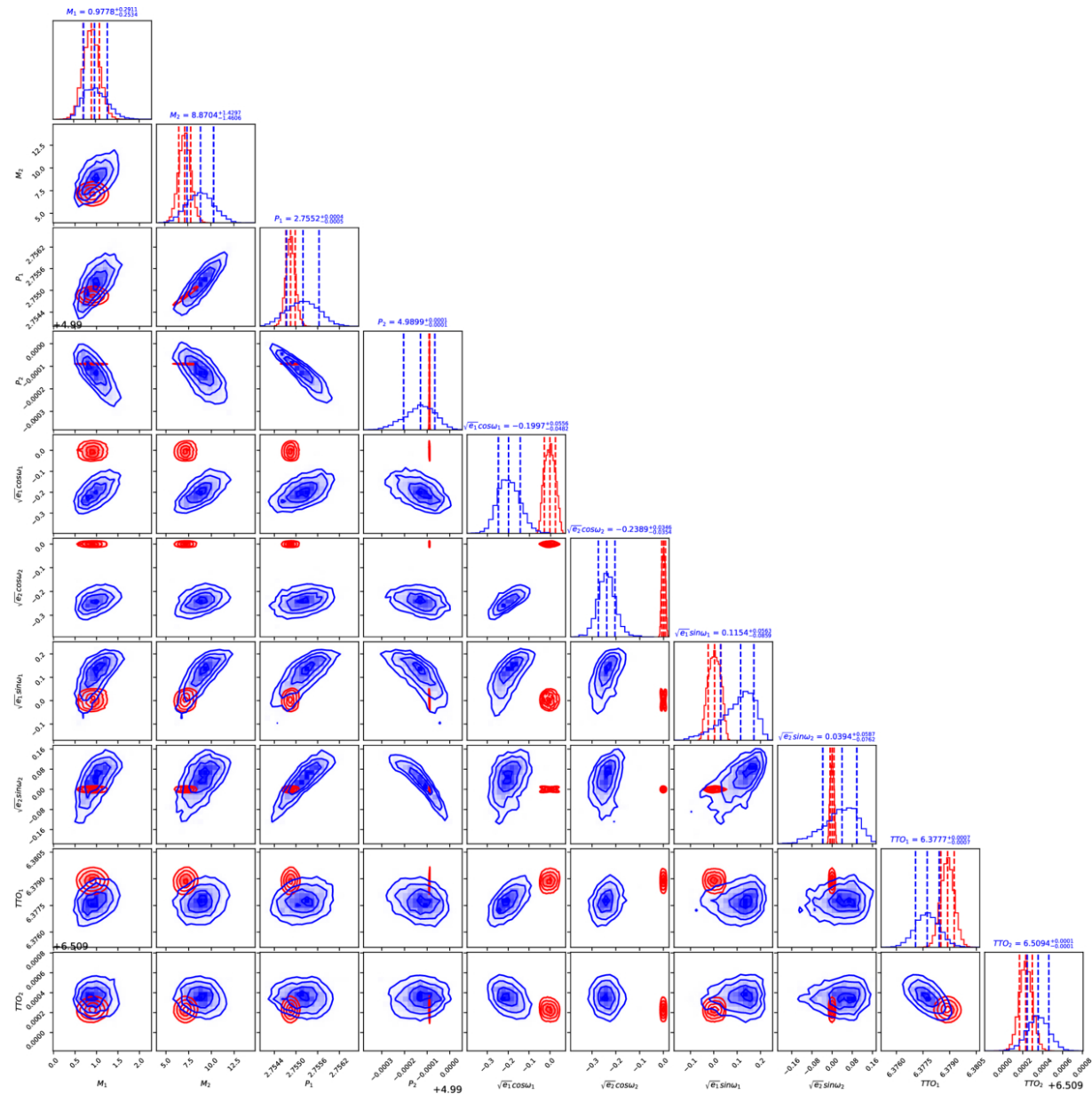
Figure 8. from Michael Greklek-McKeon et al 2025 Astron. J. 170 doi:10.3847/1538-3881/addf2d https://dx.doi.org/10.3847/1538-3881/addf2d © 2025. The Author(s). Published by the American Astronomical Society.
