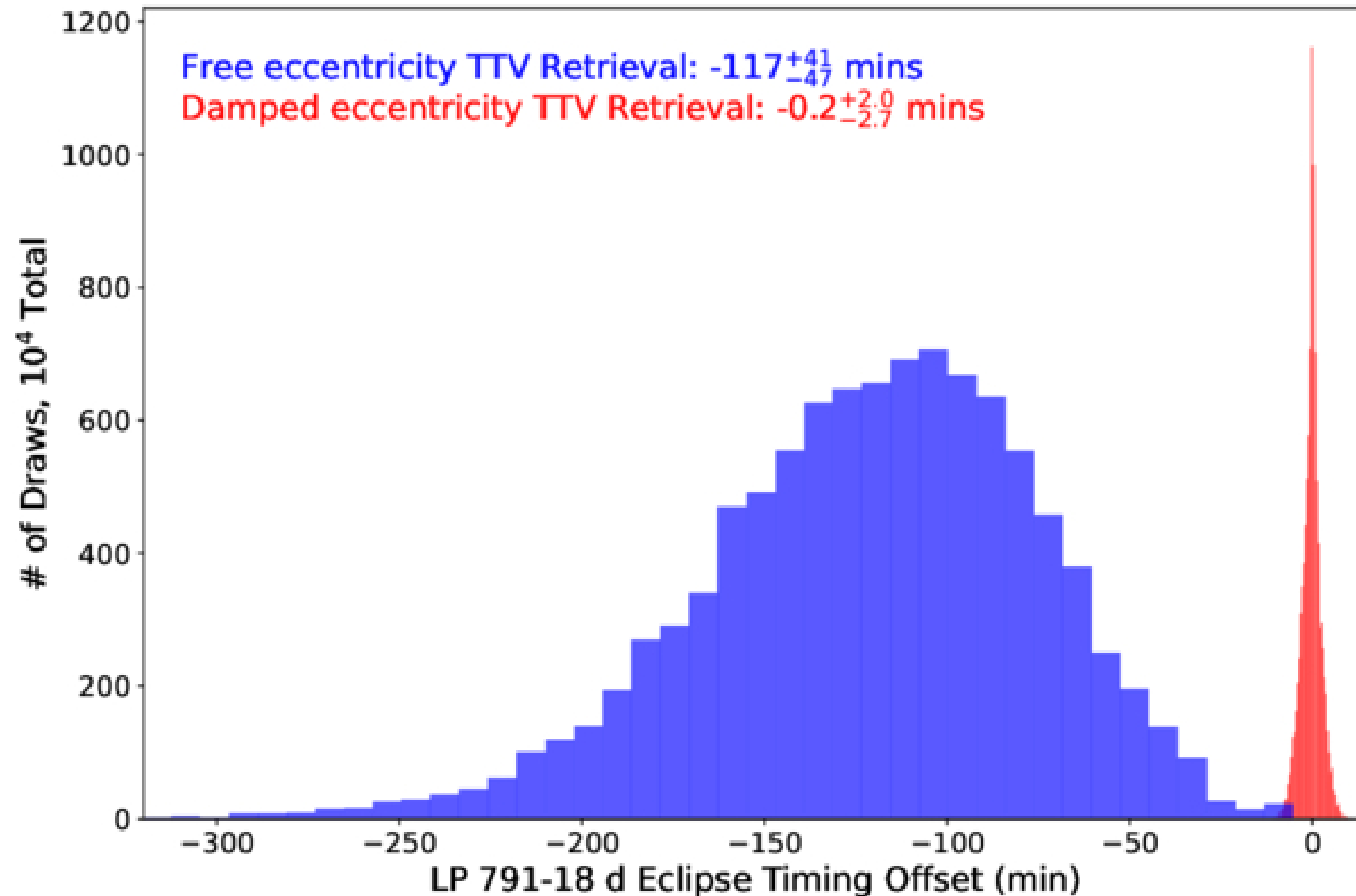
Figure 6. from Michael Greklek-McKeon et al 2025 Astron. J. 170 doi:10.3847/1538-3881/addf2d https://dx.doi.org/10.3847/1538-3881/addf2d © 2025. The Author(s). Published by the American Astronomical Society.
