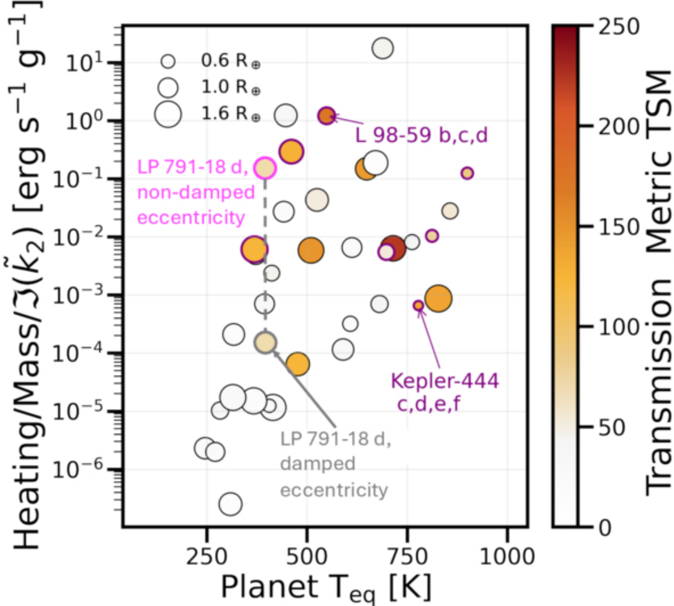
Figure 5. from Michael Greklek-McKeon et al 2025 Astron. J. 170 doi:10.3847/1538-3881/addf2d https://dx.doi.org/10.3847/1538-3881/addf2d © 2025. The Author(s). Published by the American Astronomical Society.
