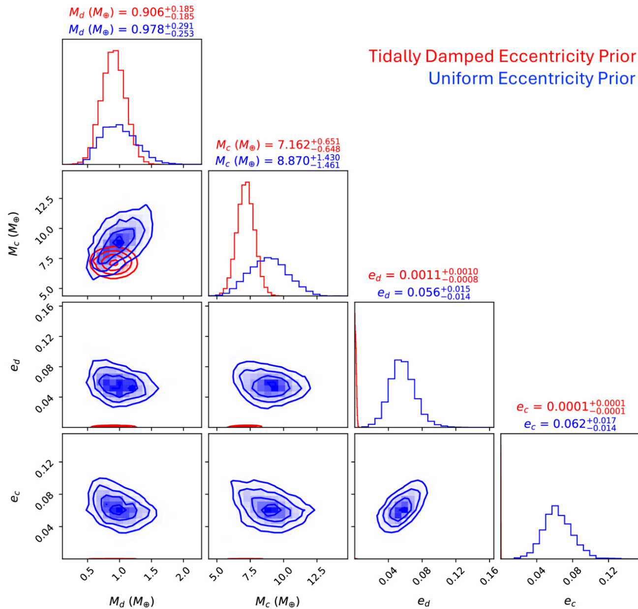
Figure 4. from Michael Greklek-McKeon et al 2025 Astron. J. 170 doi:10.3847/1538-3881/addf2d https://dx.doi.org/10.3847/1538-3881/addf2d © 2025. The Author(s). Published by the American Astronomical Society.
