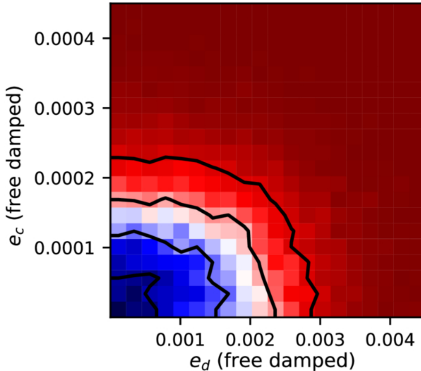
Figure 2. from Michael Greklek-McKeon et al 2025 Astron. J. 170 doi:10.3847/1538-3881/addf2d https://dx.doi.org/10.3847/1538-3881/addf2d © 2025. The Author(s). Published by the American Astronomical Society.
