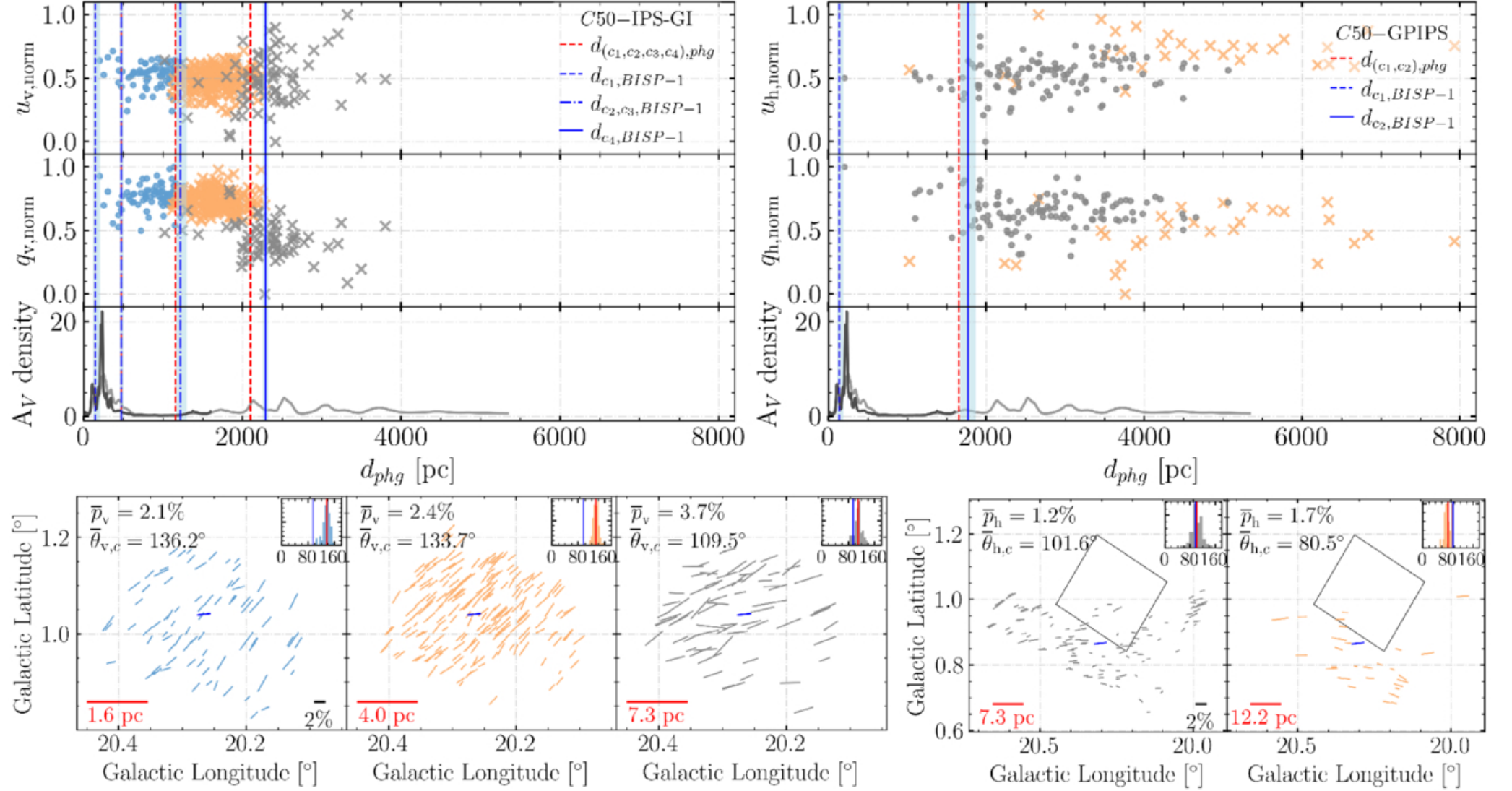
Figure 10. from Y. Angarita et al 2025 Astron. J. 170 doi:10.3847/1538-3881/addecc https://dx.doi.org/10.3847/1538-3881/addecc © 2025. The Author(s). Published by the American Astronomical Society.
