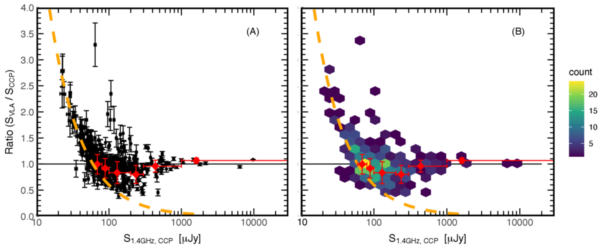
Figure 9. from Hansung B. Gim et al 2025 Astron. J. 170 doi:10.3847/1538-3881/adde56 https://dx.doi.org/10.3847/1538-3881/adde56 © 2025. The Author(s). Published by the American Astronomical Society.
