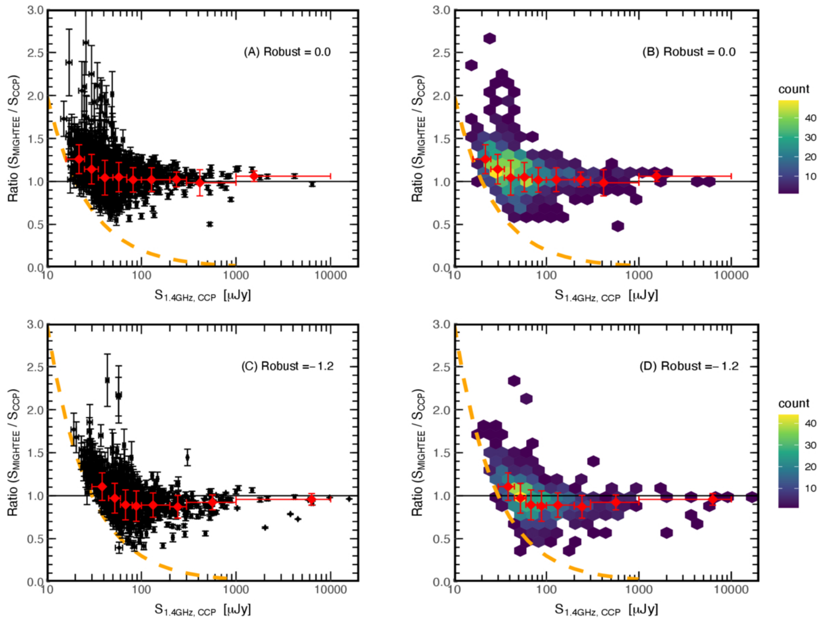
Figure 8. from Hansung B. Gim et al 2025 Astron. J. 170 doi:10.3847/1538-3881/adde56 https://dx.doi.org/10.3847/1538-3881/adde56 © 2025. The Author(s). Published by the American Astronomical Society.
