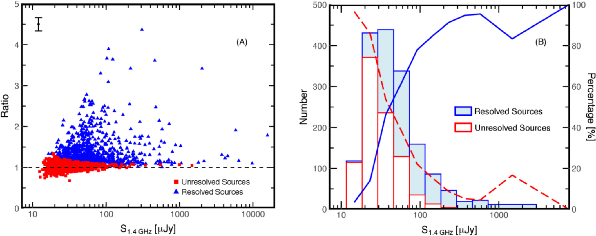
Figure 4. from Hansung B. Gim et al 2025 Astron. J. 170 doi:10.3847/1538-3881/adde56 https://dx.doi.org/10.3847/1538-3881/adde56 © 2025. The Author(s). Published by the American Astronomical Society.
