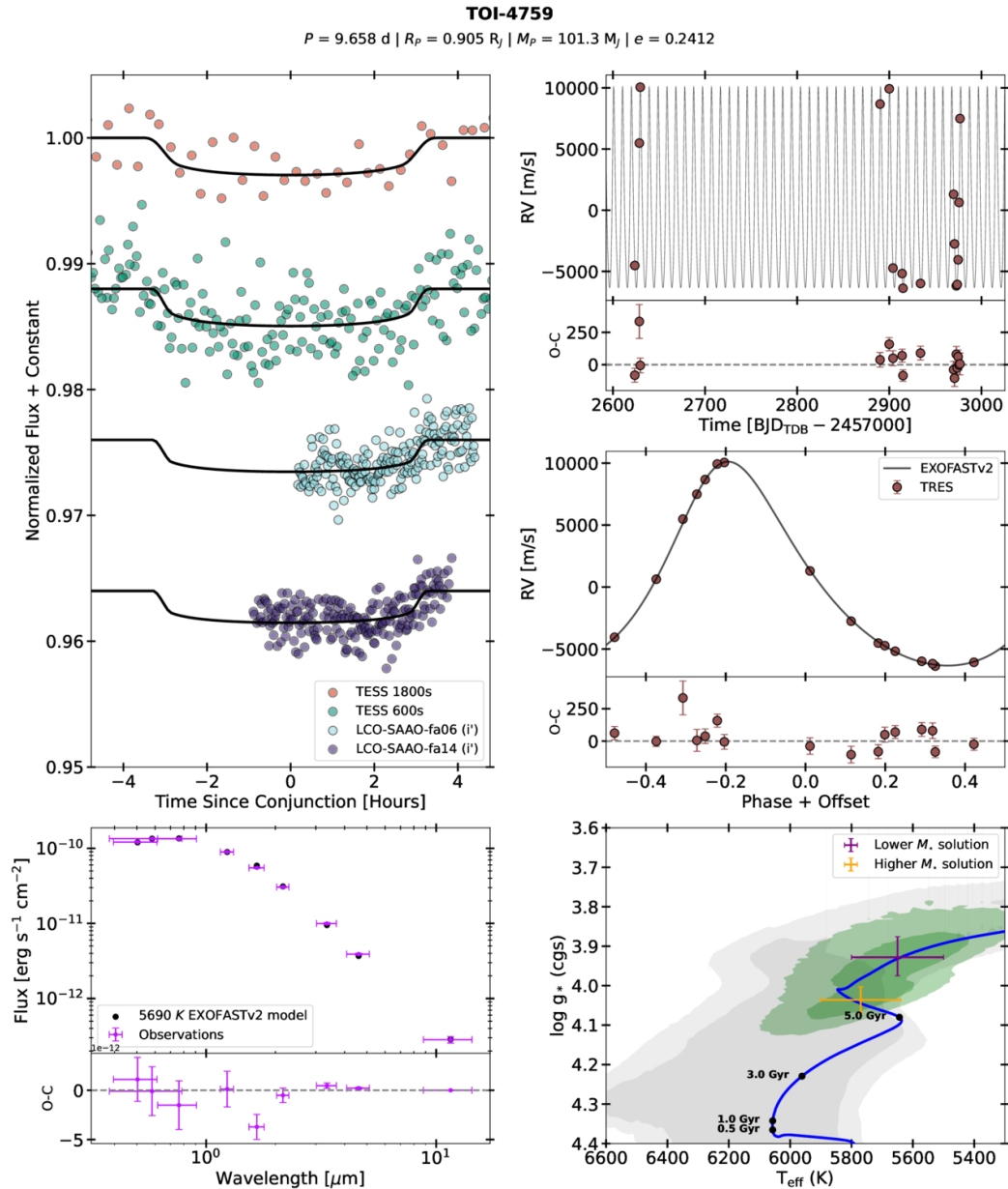
Figure 9. from Noah Vowell et al 2025 Astron. J. 170 doi:10.3847/1538-3881/addd17 https://dx.doi.org/10.3847/1538-3881/addd17 © 2025. The Author(s). Published by the American Astronomical Society.
