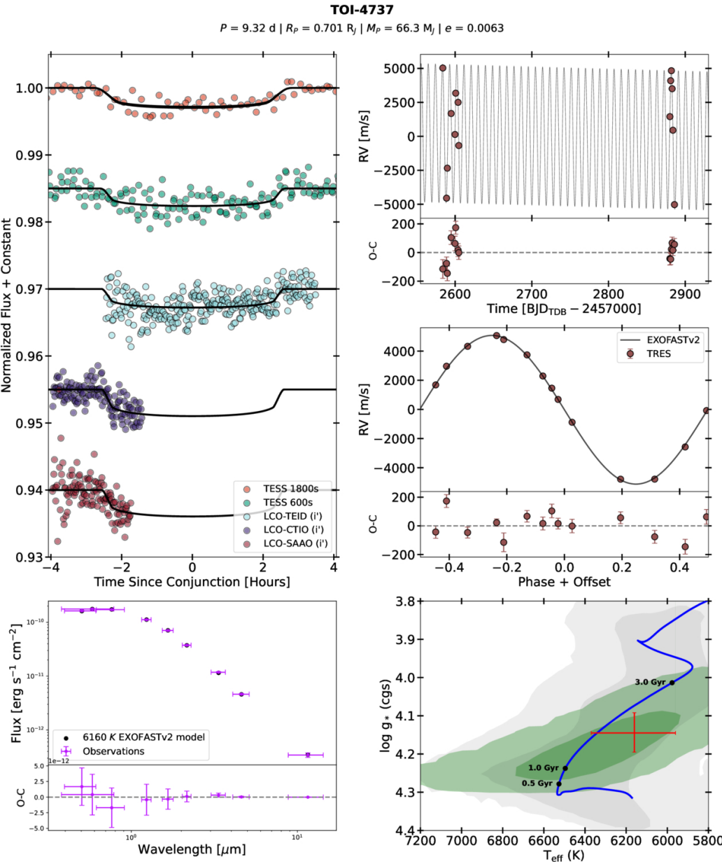
Figure 8. from Noah Vowell et al 2025 Astron. J. 170 doi:10.3847/1538-3881/addd17 https://dx.doi.org/10.3847/1538-3881/addd17 © 2025. The Author(s). Published by the American Astronomical Society.
