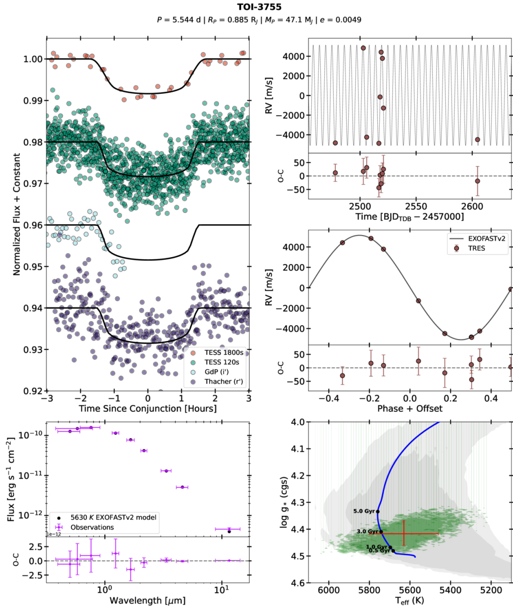
Figure 5. from Noah Vowell et al 2025 Astron. J. 170 doi:10.3847/1538-3881/addd17 https://dx.doi.org/10.3847/1538-3881/addd17 © 2025. The Author(s). Published by the American Astronomical Society.
