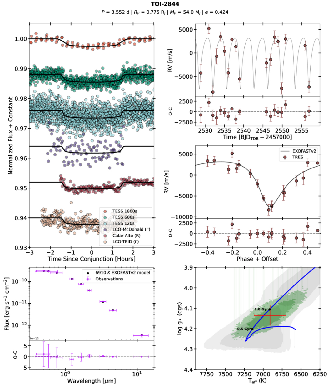
Figure 2. from Noah Vowell et al 2025 Astron. J. 170 doi:10.3847/1538-3881/addd17 https://dx.doi.org/10.3847/1538-3881/addd17 © 2025. The Author(s). Published by the American Astronomical Society.
