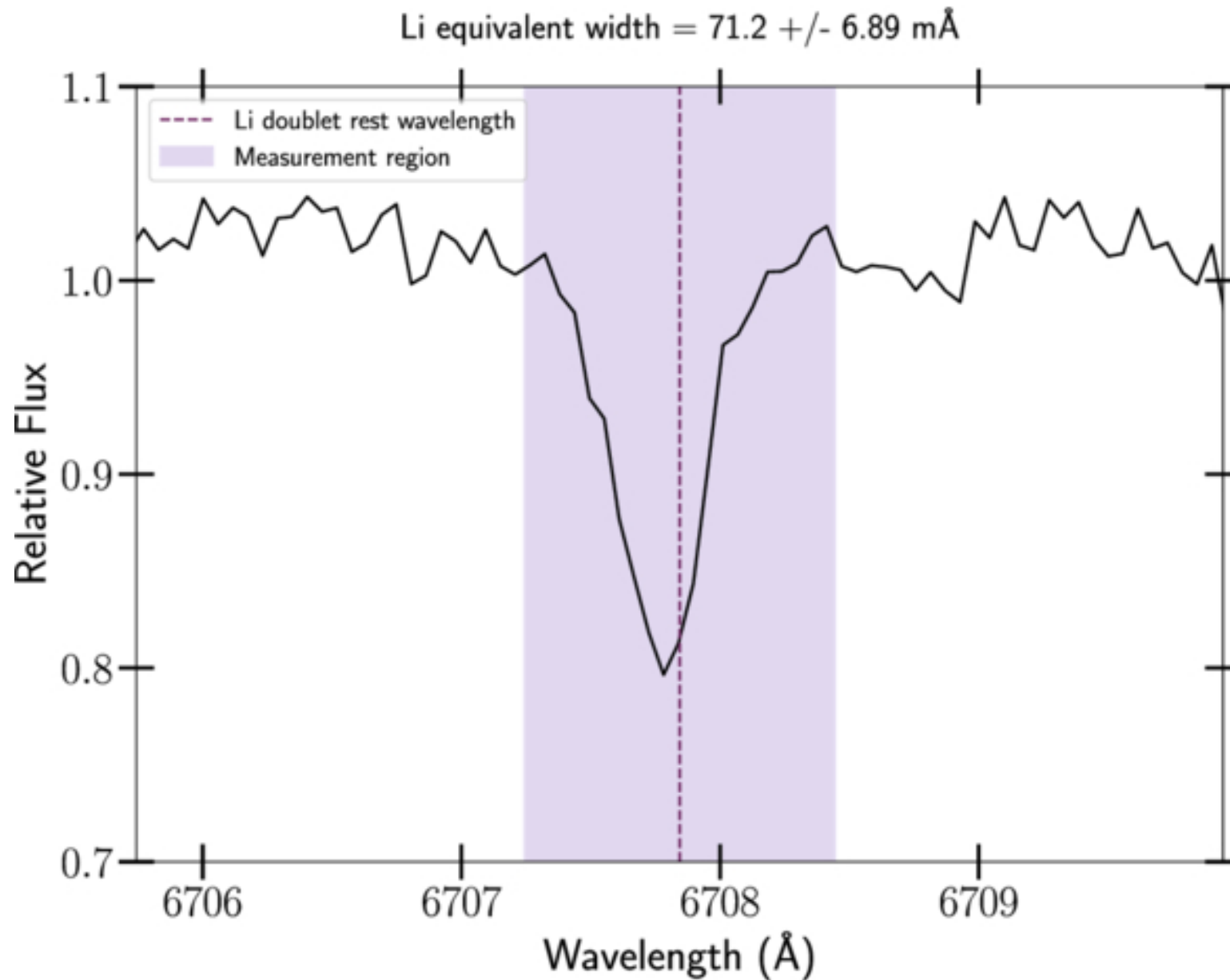
Figure 16. from Noah Vowell et al 2025 Astron. J. 170 doi:10.3847/1538-3881/addd17 https://dx.doi.org/10.3847/1538-3881/addd17 © 2025. The Author(s). Published by the American Astronomical Society.
