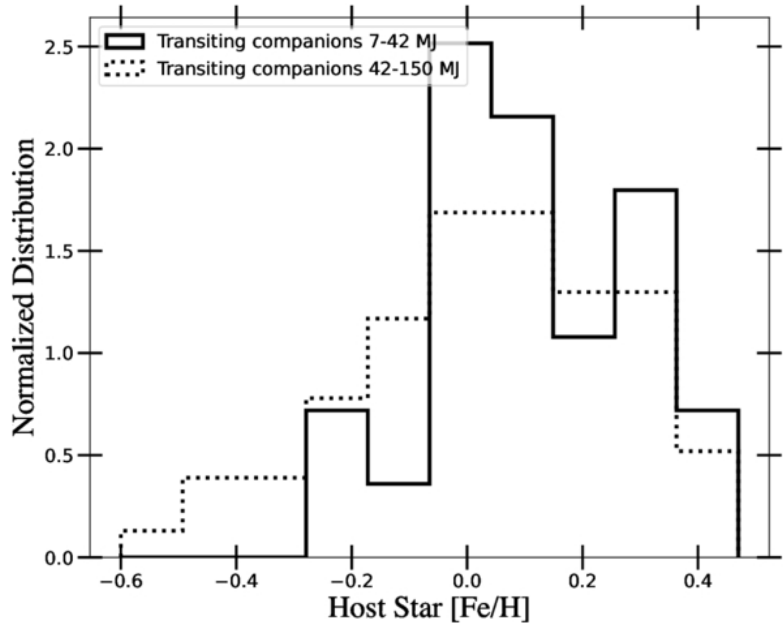
Figure 15. from Noah Vowell et al 2025 Astron. J. 170 doi:10.3847/1538-3881/addd17 https://dx.doi.org/10.3847/1538-3881/addd17 © 2025. The Author(s). Published by the American Astronomical Society.
