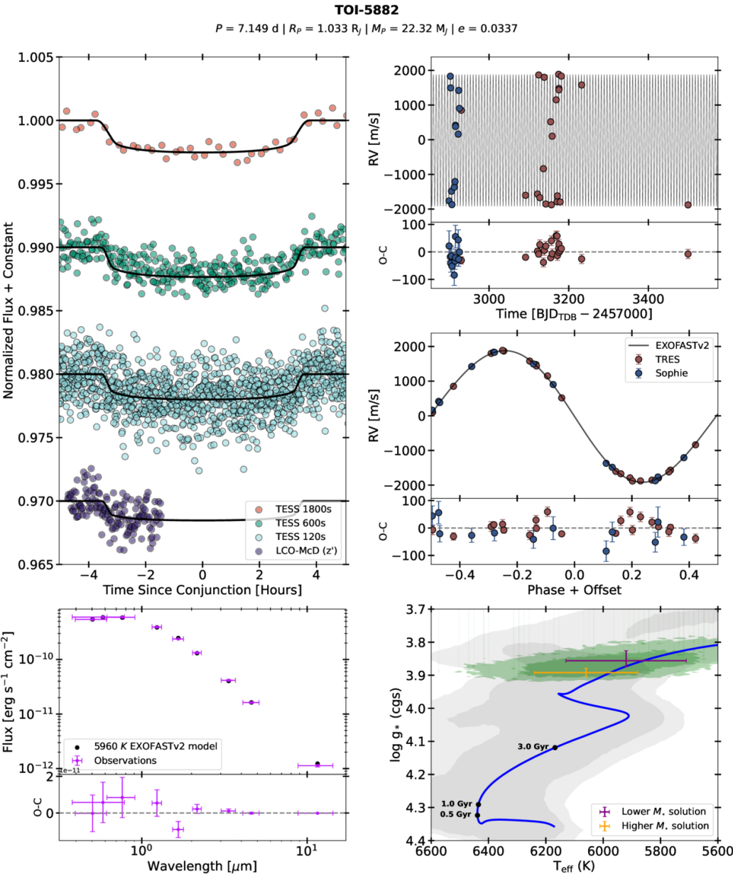
Figure 12. from Noah Vowell et al 2025 Astron. J. 170 doi:10.3847/1538-3881/addd17 https://dx.doi.org/10.3847/1538-3881/addd17 © 2025. The Author(s). Published by the American Astronomical Society.
