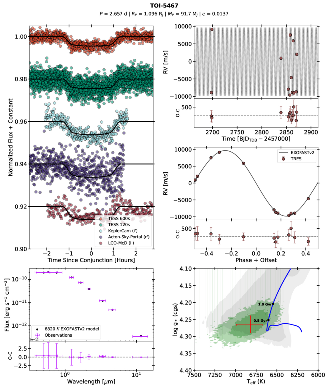
Figure 11. from Noah Vowell et al 2025 Astron. J. 170 doi:10.3847/1538-3881/addd17 https://dx.doi.org/10.3847/1538-3881/addd17 © 2025. The Author(s). Published by the American Astronomical Society.
