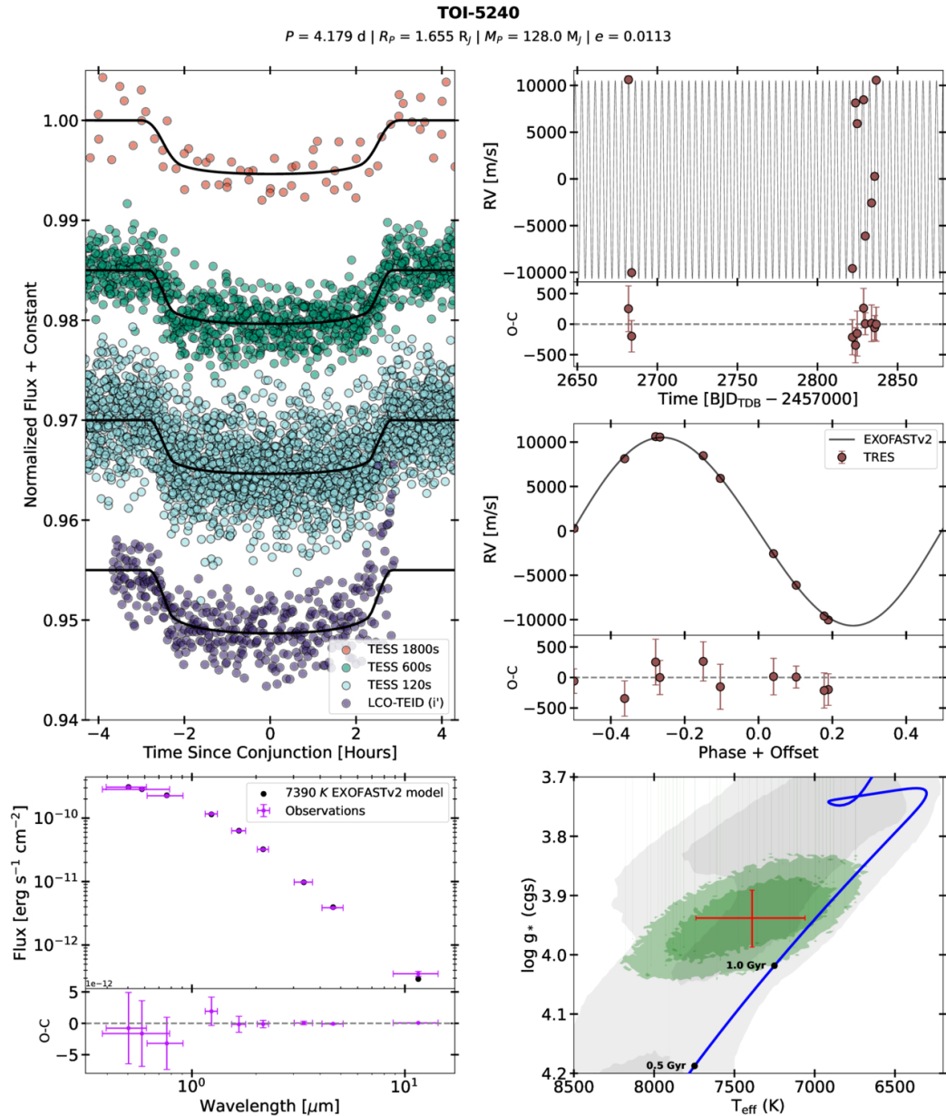
Figure 10. from Noah Vowell et al 2025 Astron. J. 170 doi:10.3847/1538-3881/addd17 https://dx.doi.org/10.3847/1538-3881/addd17 © 2025. The Author(s). Published by the American Astronomical Society.
