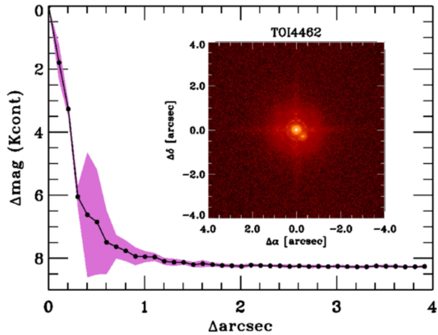
Figure 1. from Noah Vowell et al 2025 Astron. J. 170 doi:10.3847/1538-3881/addd17 https://dx.doi.org/10.3847/1538-3881/addd17 © 2025. The Author(s). Published by the American Astronomical Society.
