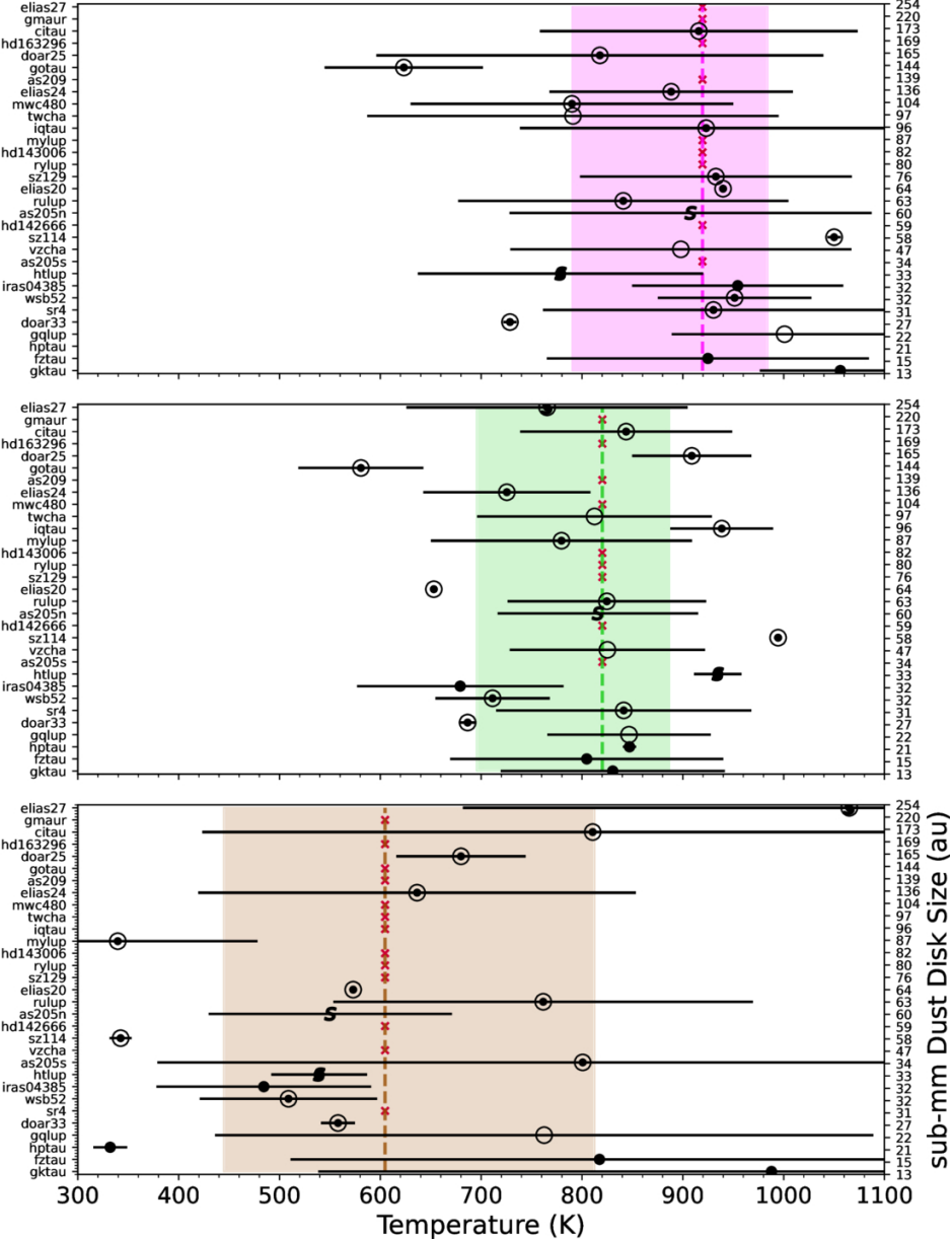
Figure 9. from Nicole Arulanantham et al 2025 Astron. J. 170 doi:10.3847/1538-3881/addd01 https://dx.doi.org/10.3847/1538-3881/addd01 © 2025. The Author(s). Published by the American Astronomical Society.
