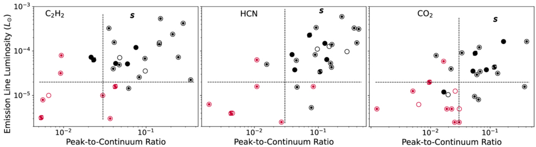
Figure 8. from Nicole Arulanantham et al 2025 Astron. J. 170 doi:10.3847/1538-3881/addd01 https://dx.doi.org/10.3847/1538-3881/addd01 © 2025. The Author(s). Published by the American Astronomical Society.
