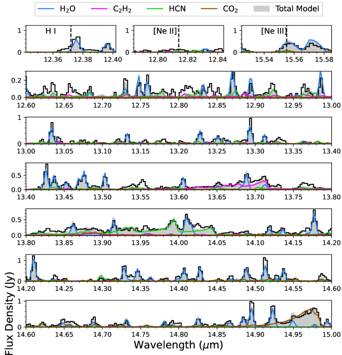
Figure 7. from Nicole Arulanantham et al 2025 Astron. J. 170 doi:10.3847/1538-3881/addd01 https://dx.doi.org/10.3847/1538-3881/addd01 © 2025. The Author(s). Published by the American Astronomical Society.
